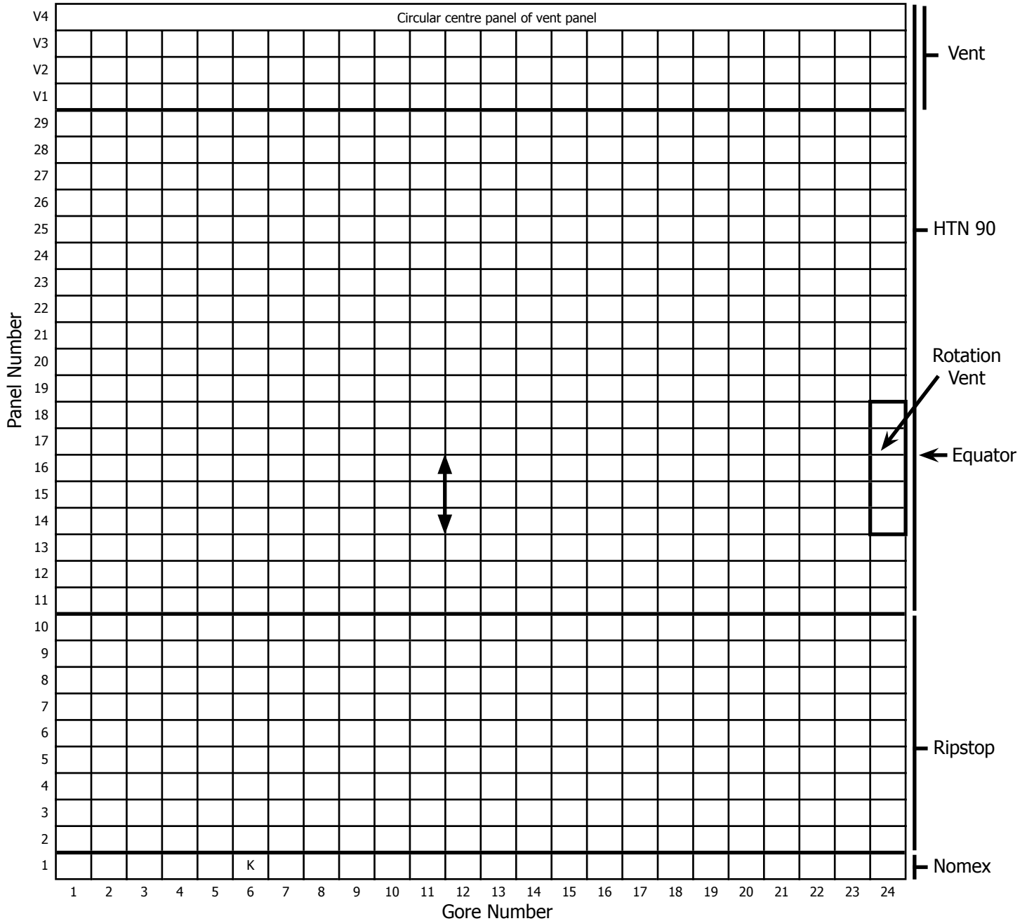
Vent Panel
