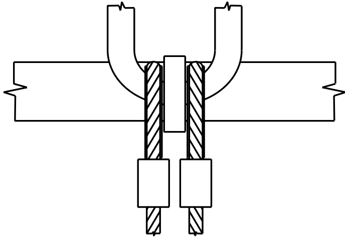
Connection of basket Attachment Points
