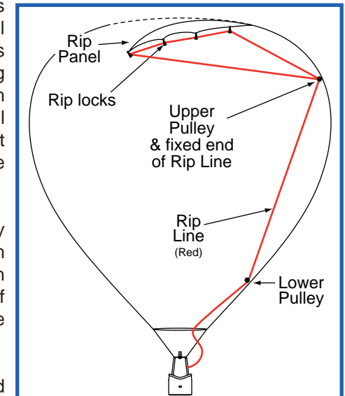
• Circular Velcro Rip Panel
