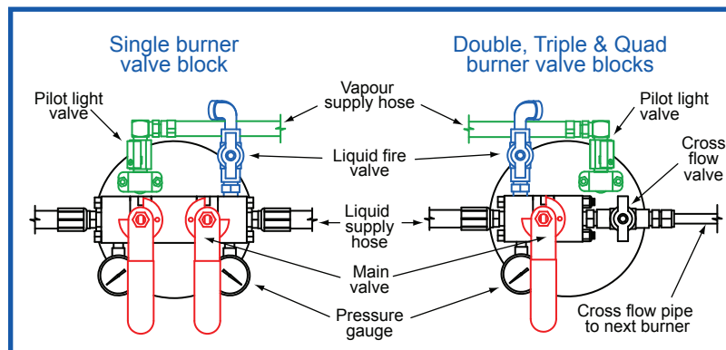
• Series 3 burner valve block layouts
