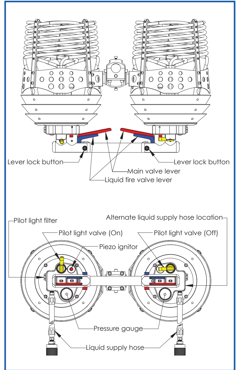
• Series 4 Valve block layout
